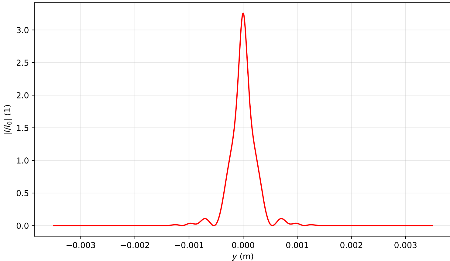
Intensity profile I(x=0, y, z=0.955)/I_0 , \text{Pin}=5.0\text{Pcr} , artificial time
